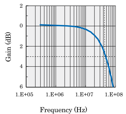
Fig6. Frequency Response
